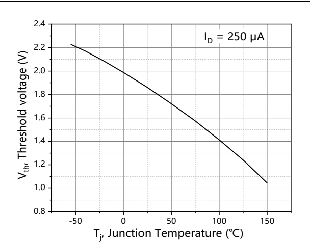
Figure 8. Threshold voltage
